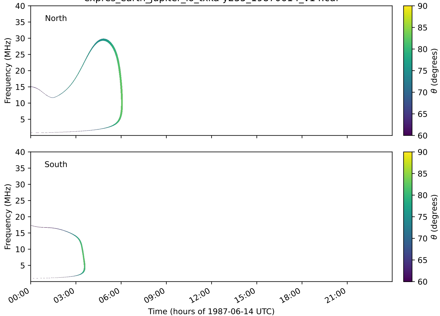
expres_earth_jupiter_io_txka-y235_19870614_v14.cdf
