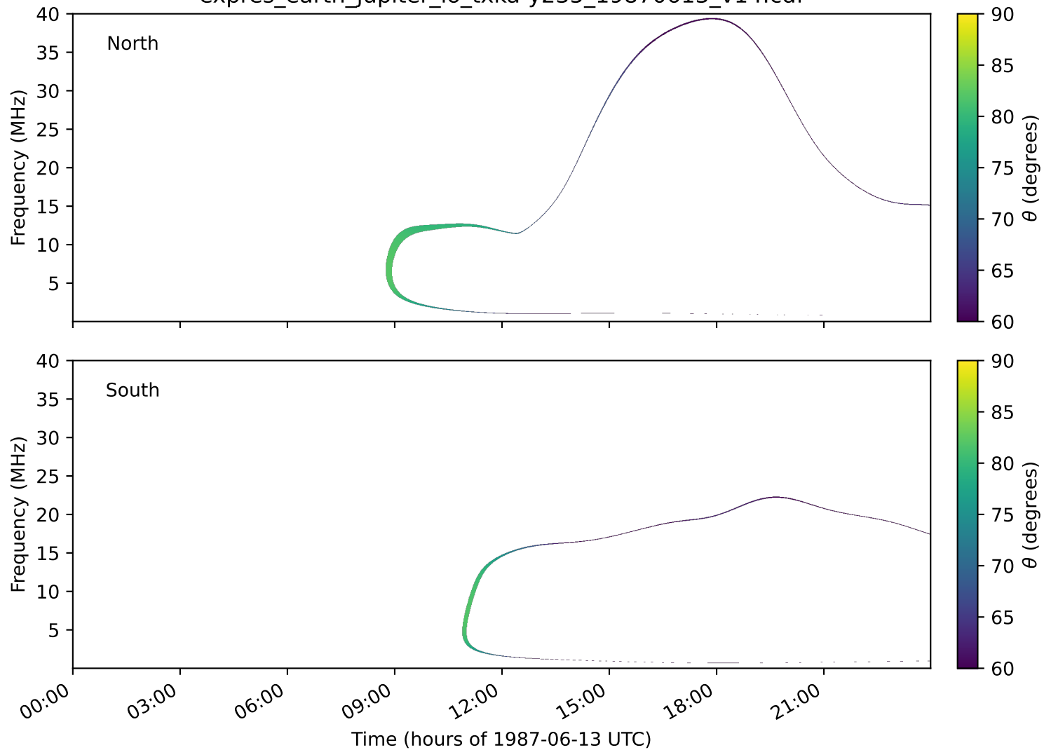
expres_earth_jupiter_io_txka-y235_19870613_v14.cdf
