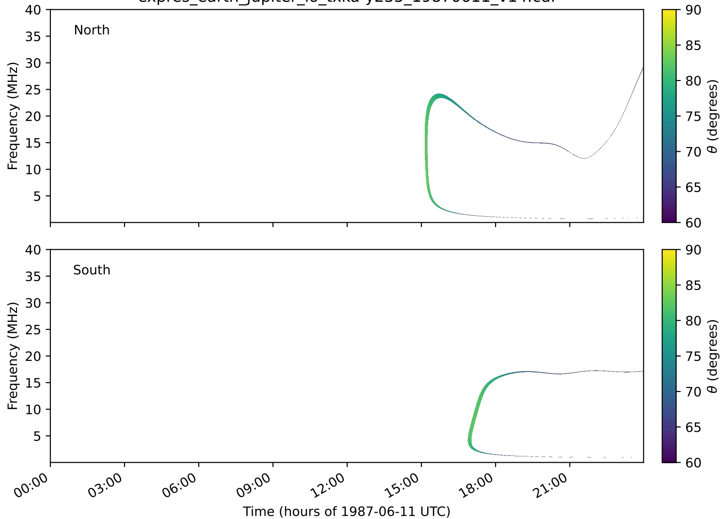
expres_earth_jupiter_io_txka-y235_19870611_v14.cdf
