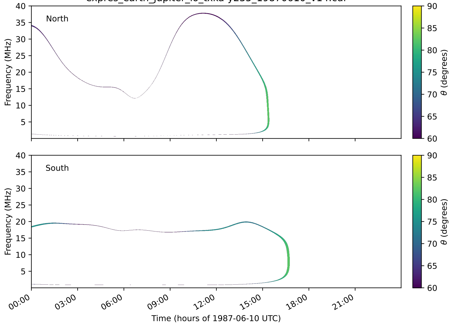
expres_earth_jupiter_io_txka-y235_19870610_v14.cdf
