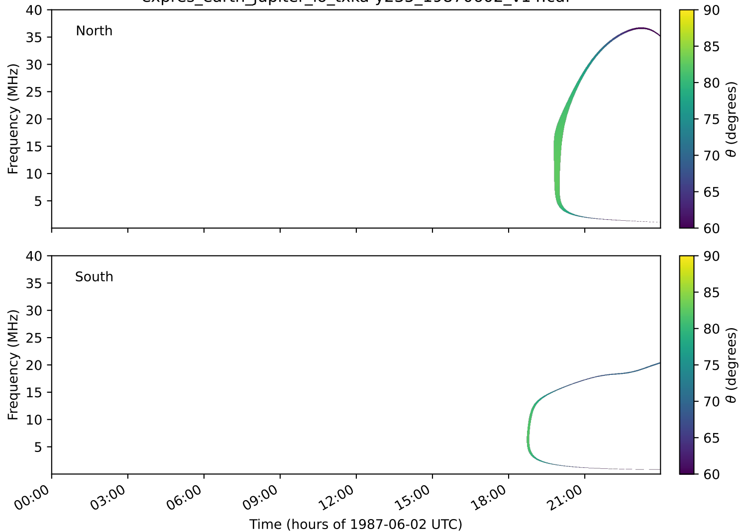
expres_earth_jupiter_io_txka-y235_19870602_v14.cdf
