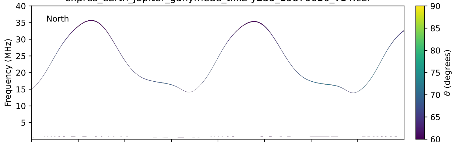
expres_earth_jupiter_ganymede_txka-y235_19870626_v14.cdf
