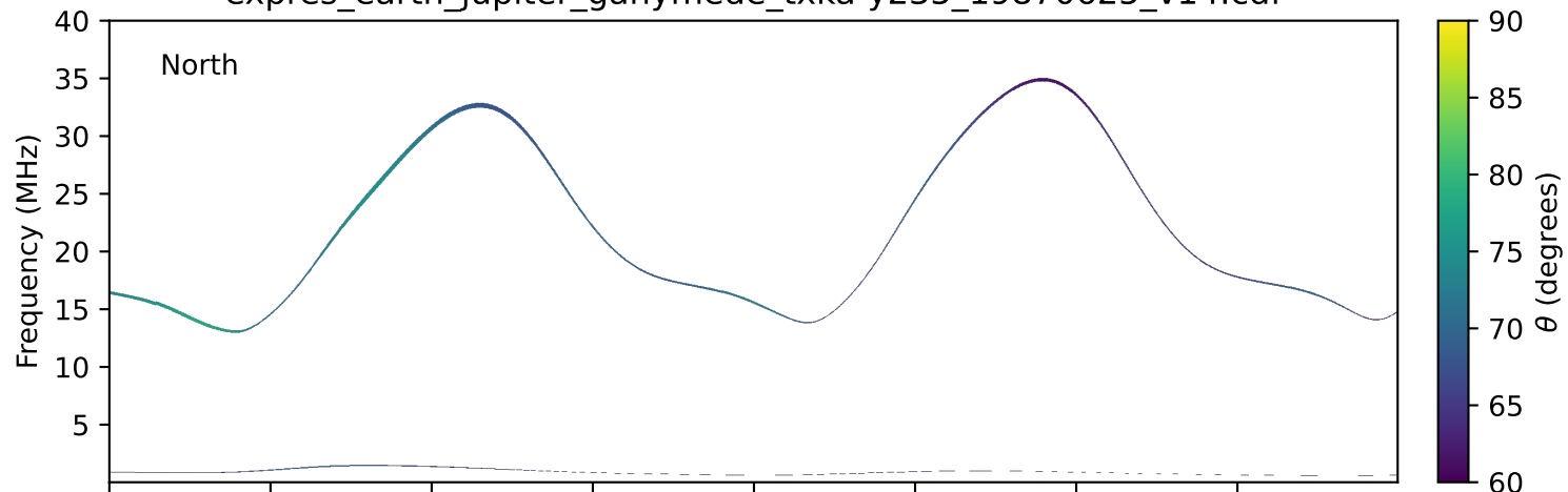
expres_earth_jupiter_ganymede_txka-y235_19870625_v14.cdf
