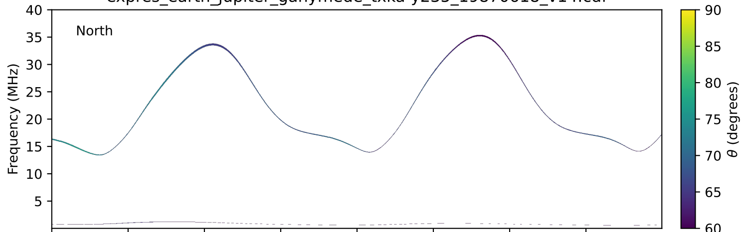
expres_earth_jupiter_ganymede_txka-y235_19870618_v14.cdf
