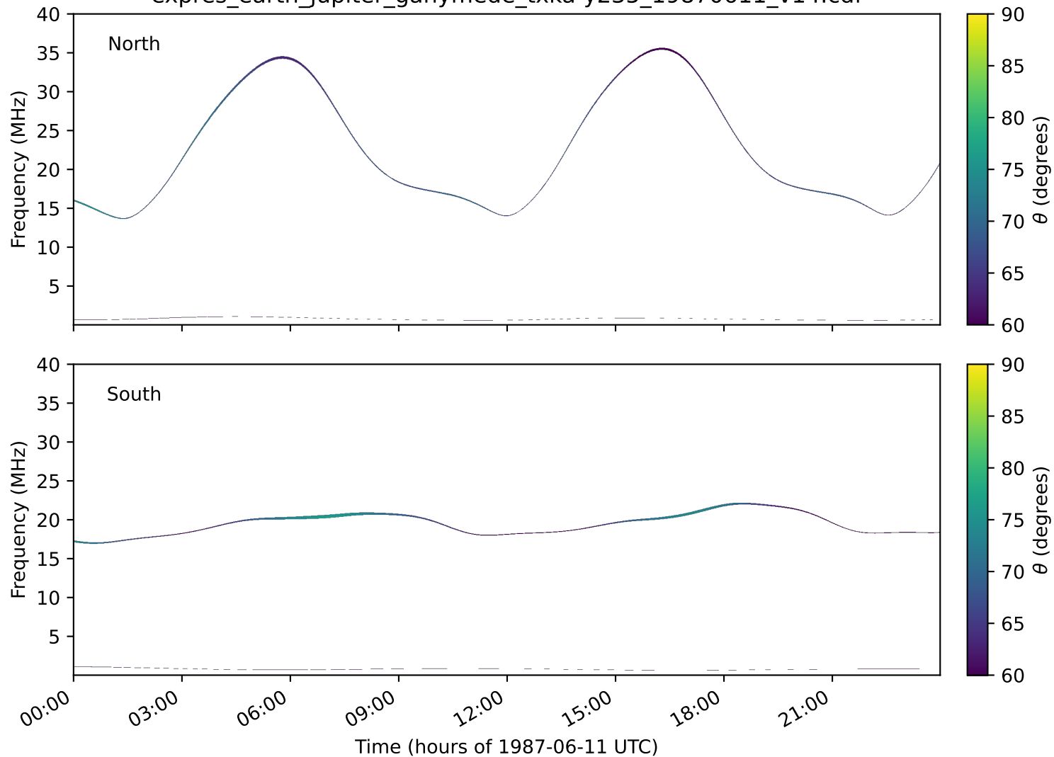
expres_earth_jupiter_ganymede_txka-y235_19870611_v14.cdf
