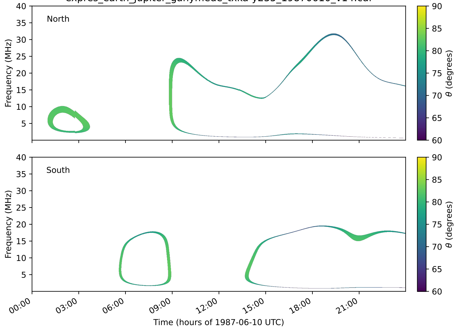
expres_earth_jupiter_ganymede_txka-y235_19870610_v14.cdf
