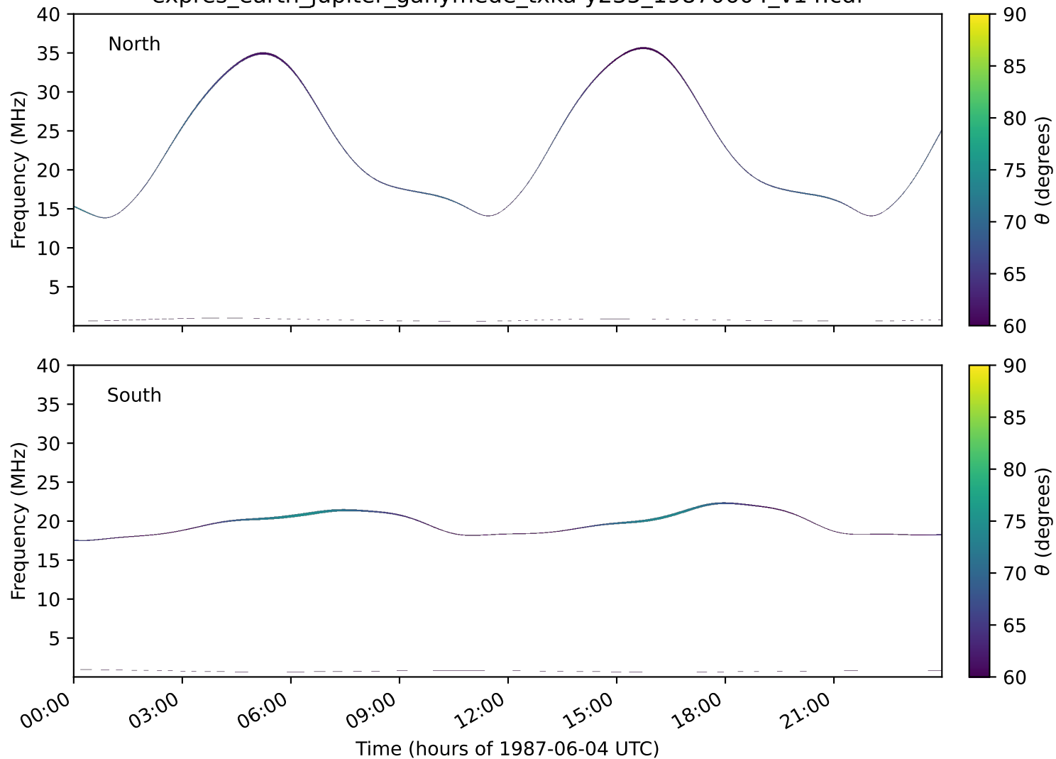
expres_earth_jupiter_ganymede_txka-y235_19870604_v14.cdf
