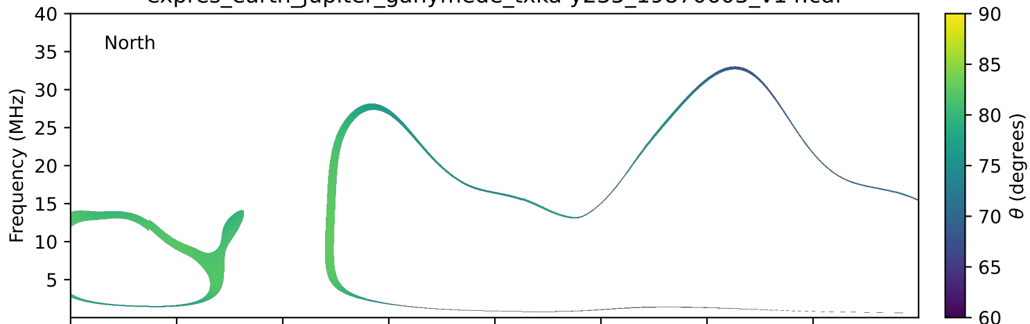
expres_earth_jupiter_ganymede_txka-y235_19870603_v14.cdf
