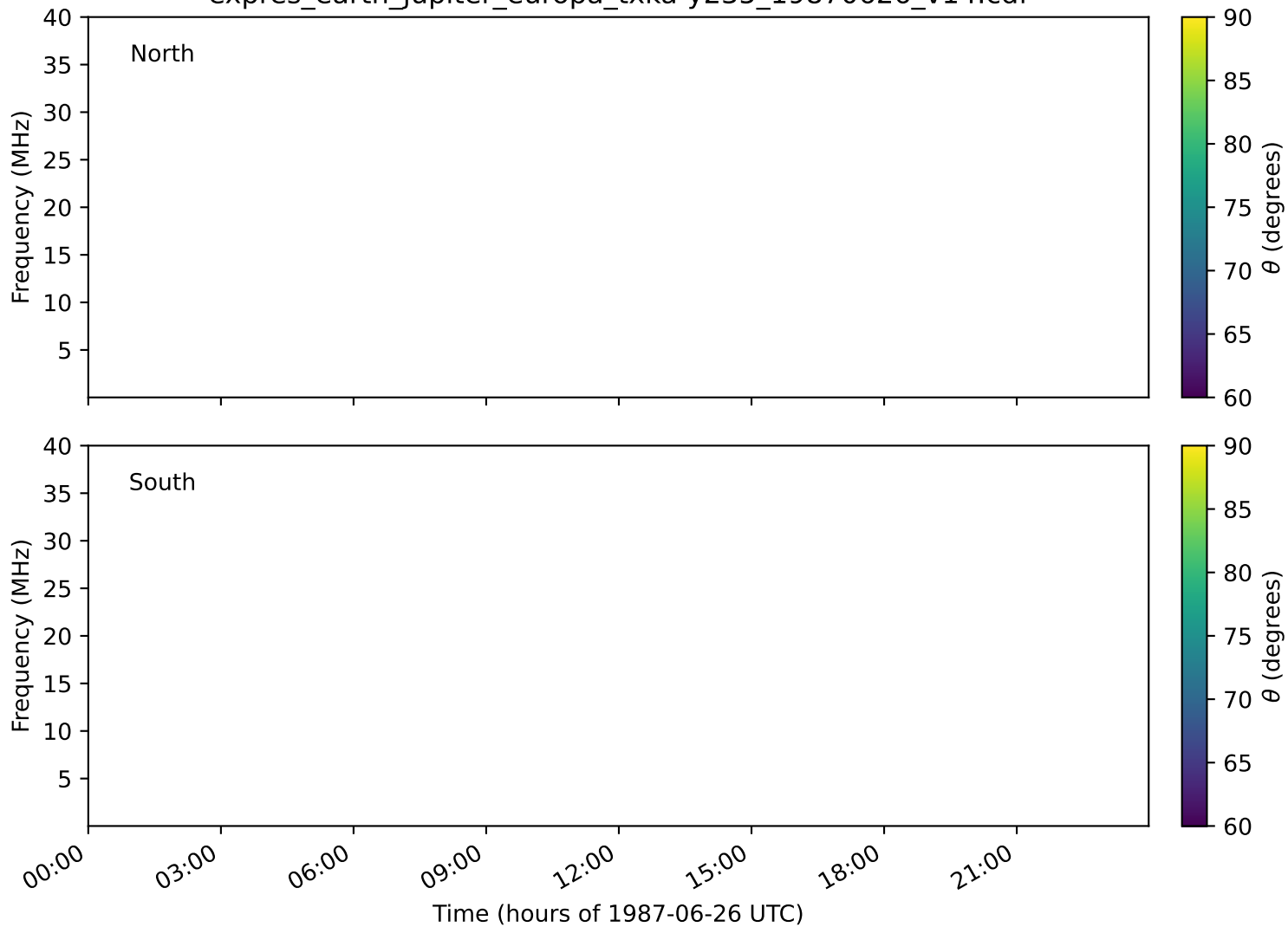
expres_earth_jupiter_europa_txka-y235_19870626_v14.cdf
