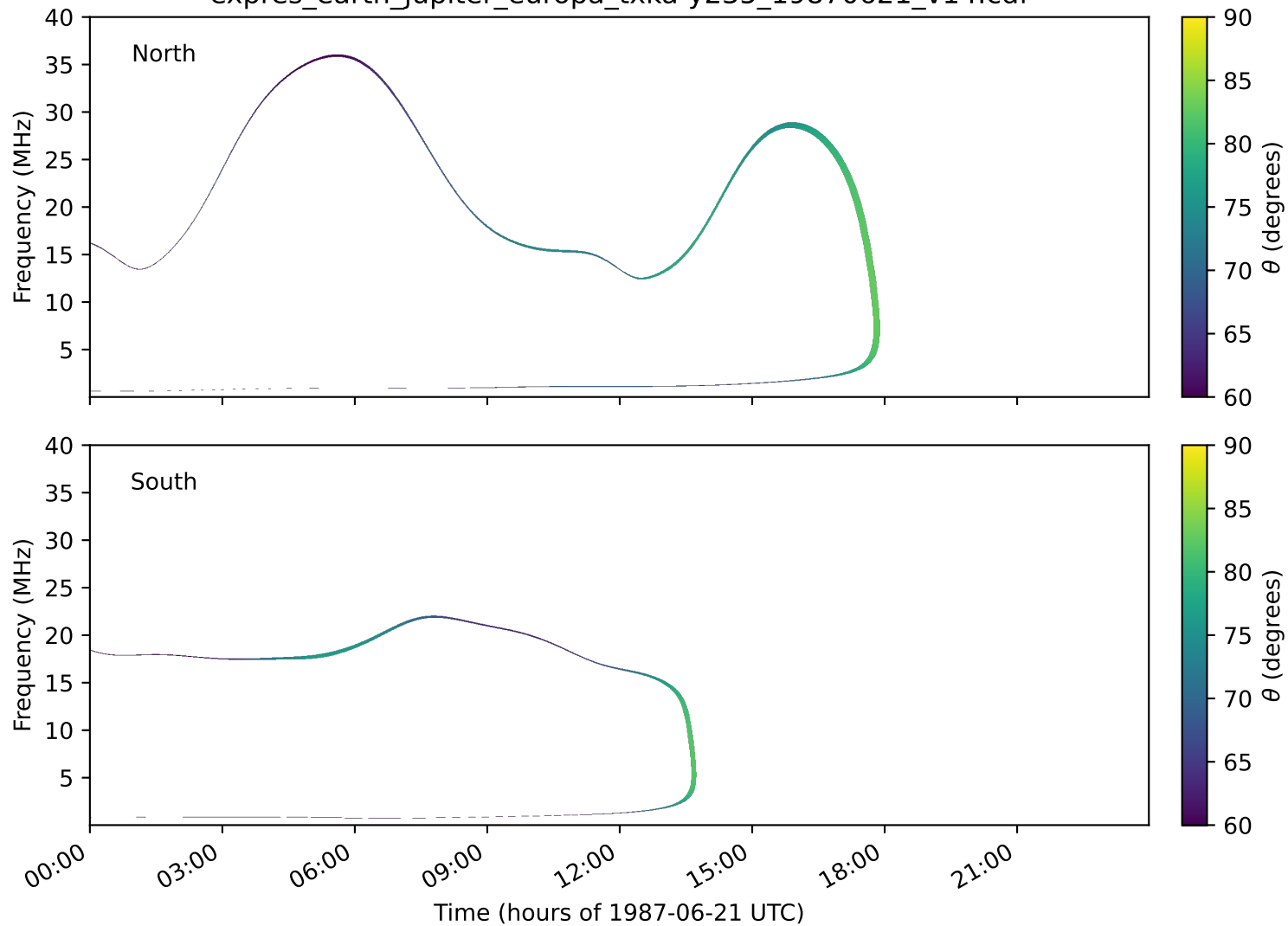
expres_earth_jupiter_europa_txka-y235_19870621_v14.cdf
