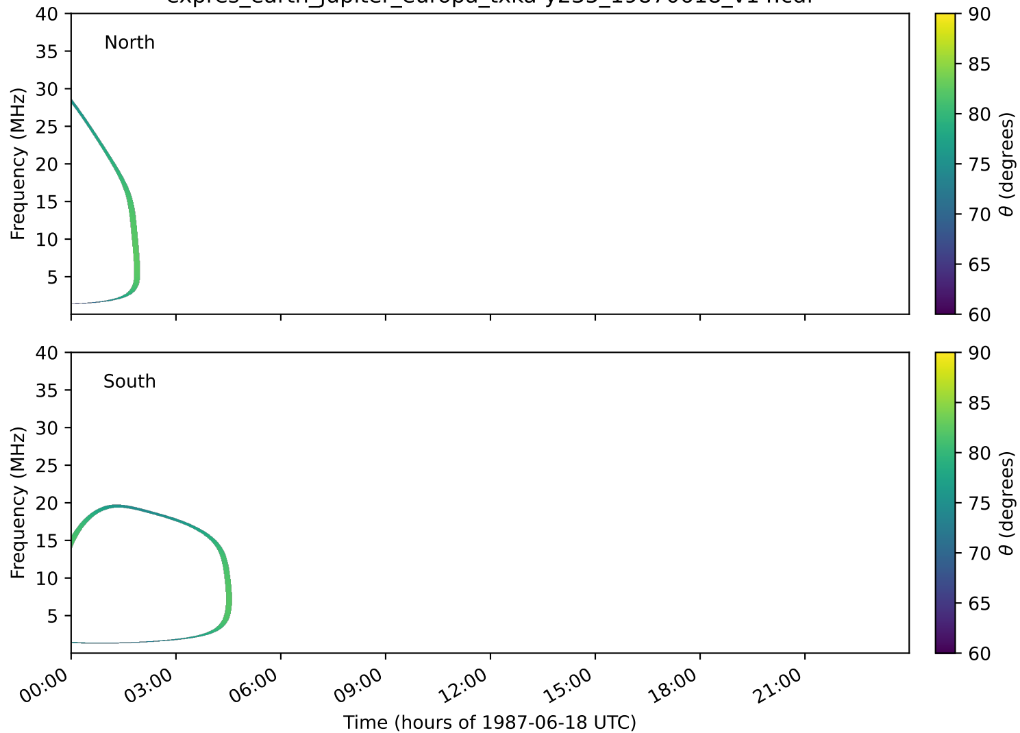
expres_earth_jupiter_europa_txka-y235_19870618_v14.cdf
