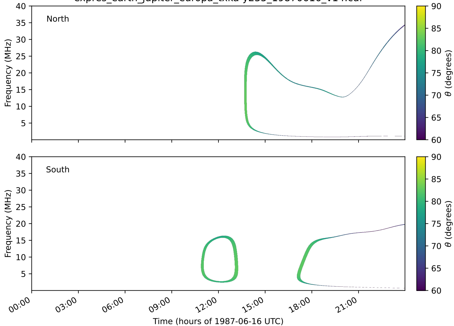
expres_earth_jupiter_europa_txka-y235_19870616_v14.cdf
