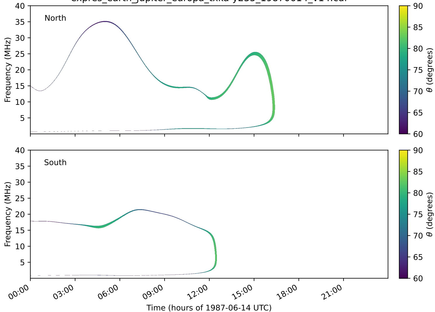
expres_earth_jupiter_europa_txka-y235_19870614_v14.cdf
