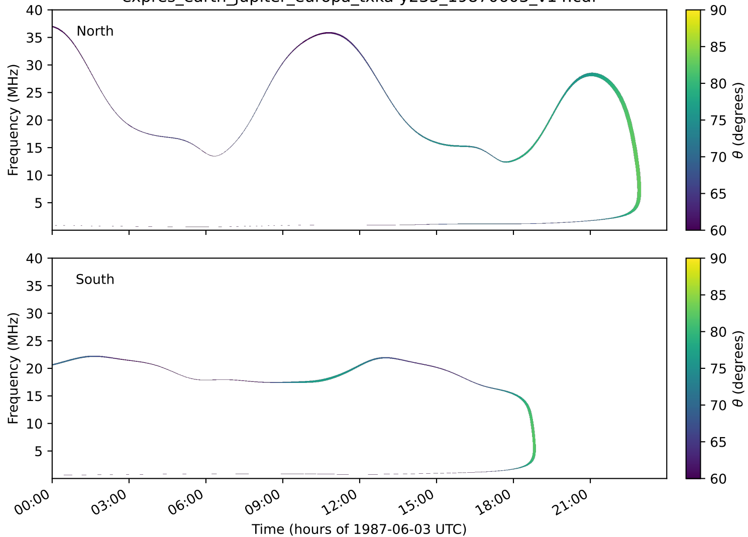
expres_earth_jupiter_europa_txka-y235_19870603_v14.cdf
