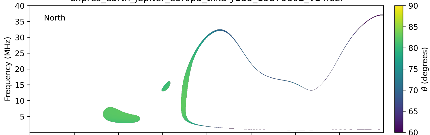
expres_earth_jupiter_europa_txka-y235_19870602_v14.cdf
