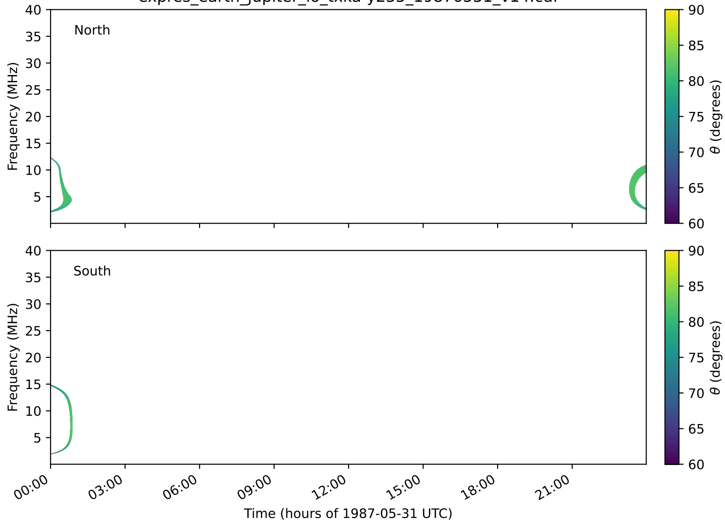
expres_earth_jupiter_io_txka-y235_19870531_v14.cdf
