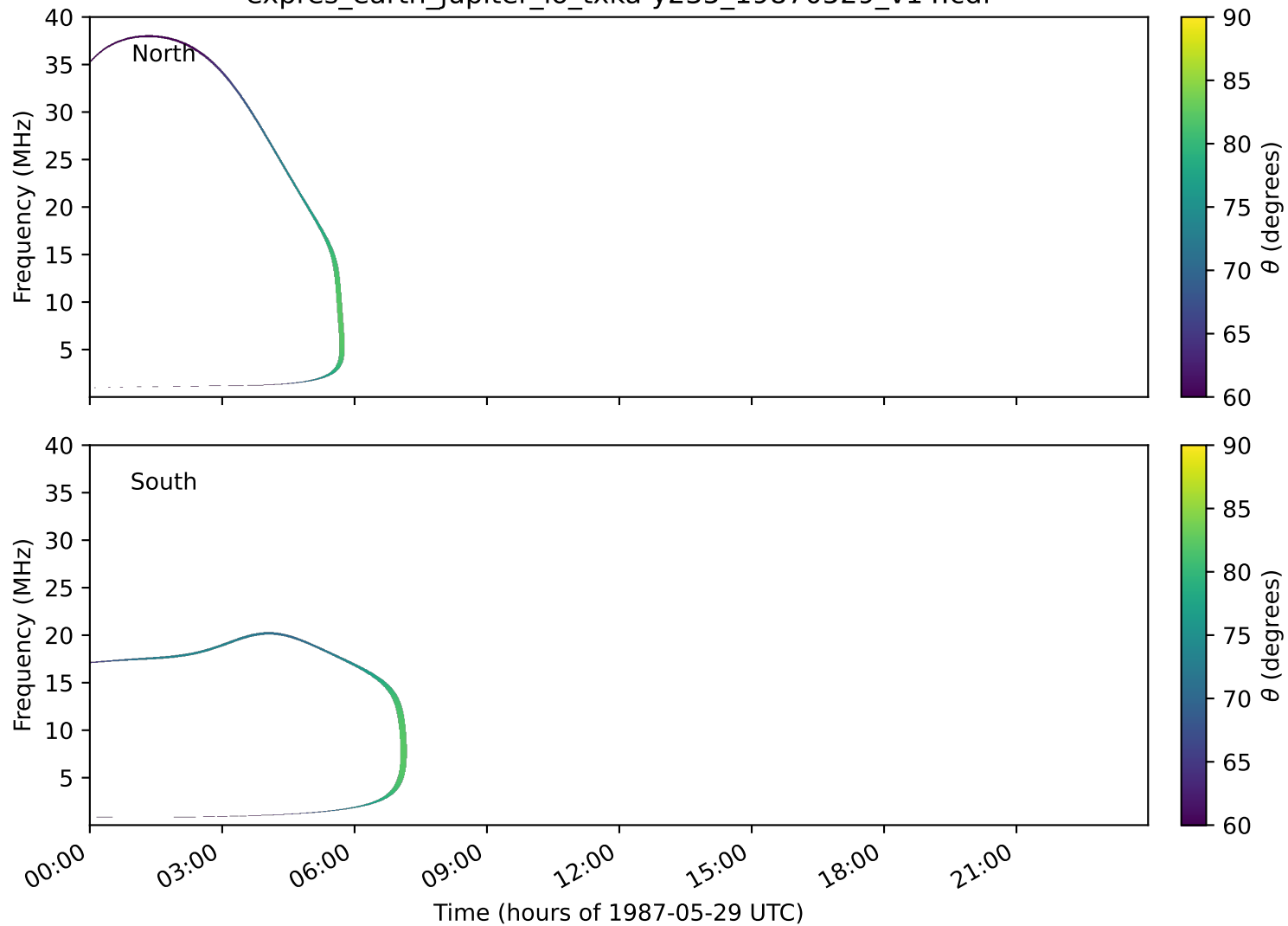
expres_earth_jupiter_io_txka-y235_19870529_v14.cdf
