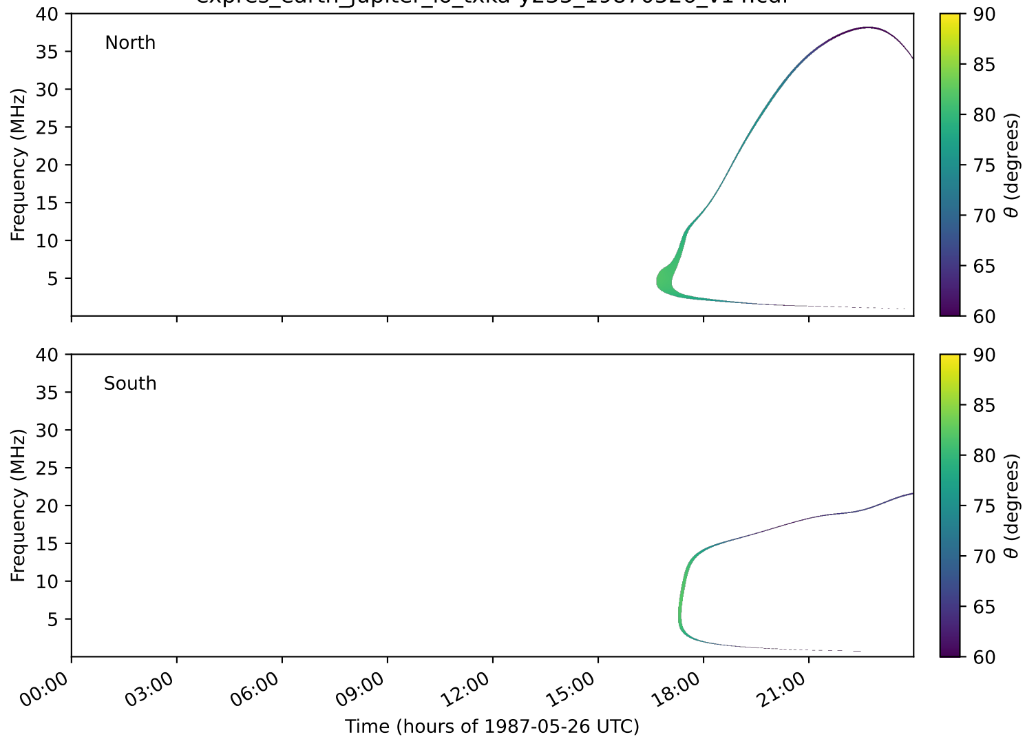
expres_earth_jupiter_io_txka-y235_19870526_v14.cdf
