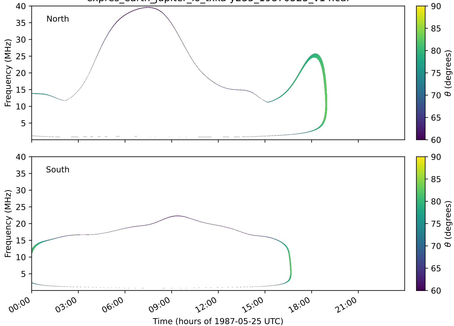
expres_earth_jupiter_io_txka-y235_19870525_v14.cdf
