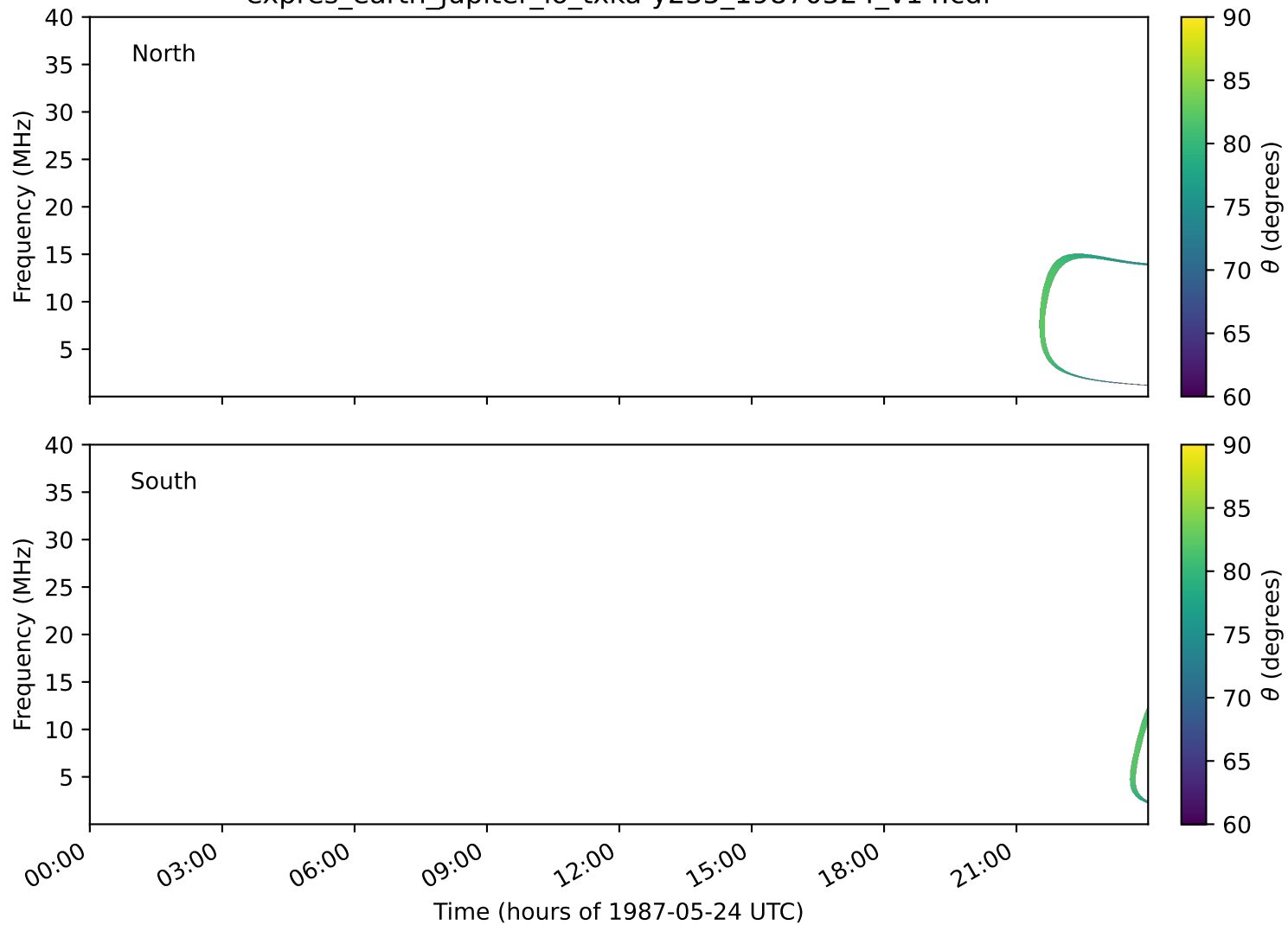
expres_earth_jupiter_io_txka-y235_19870524_v14.cdf
