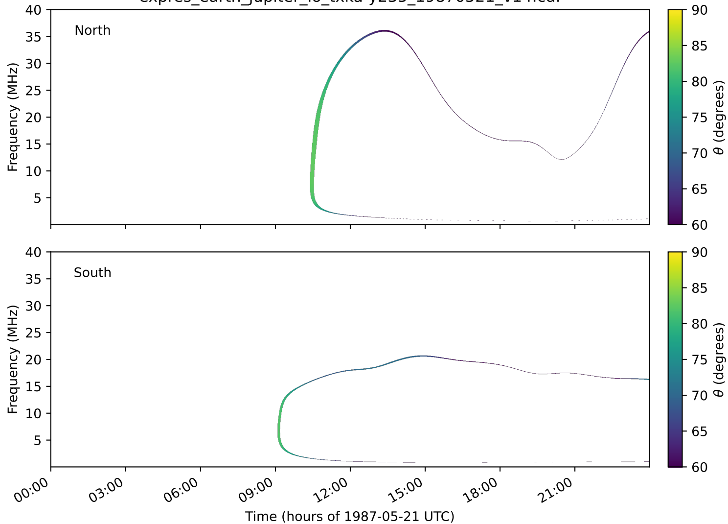
expres_earth_jupiter_io_txka-y235_19870521_v14.cdf
