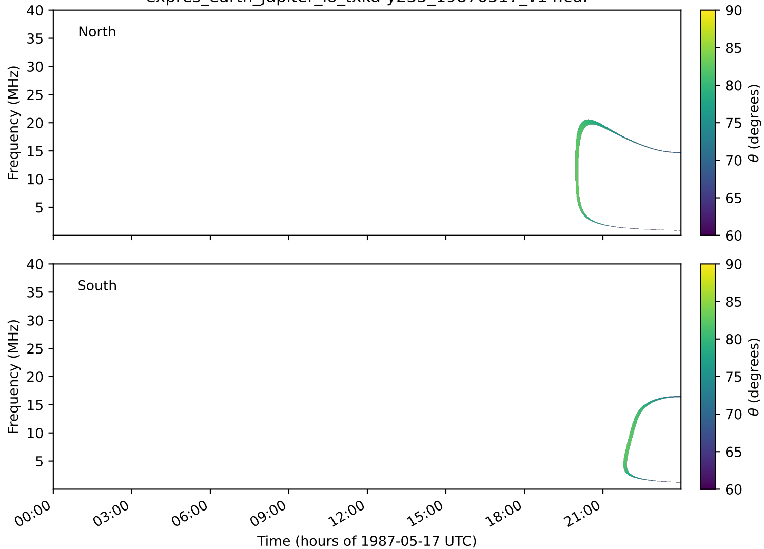
expres_earth_jupiter_io_txka-y235_19870517_v14.cdf
