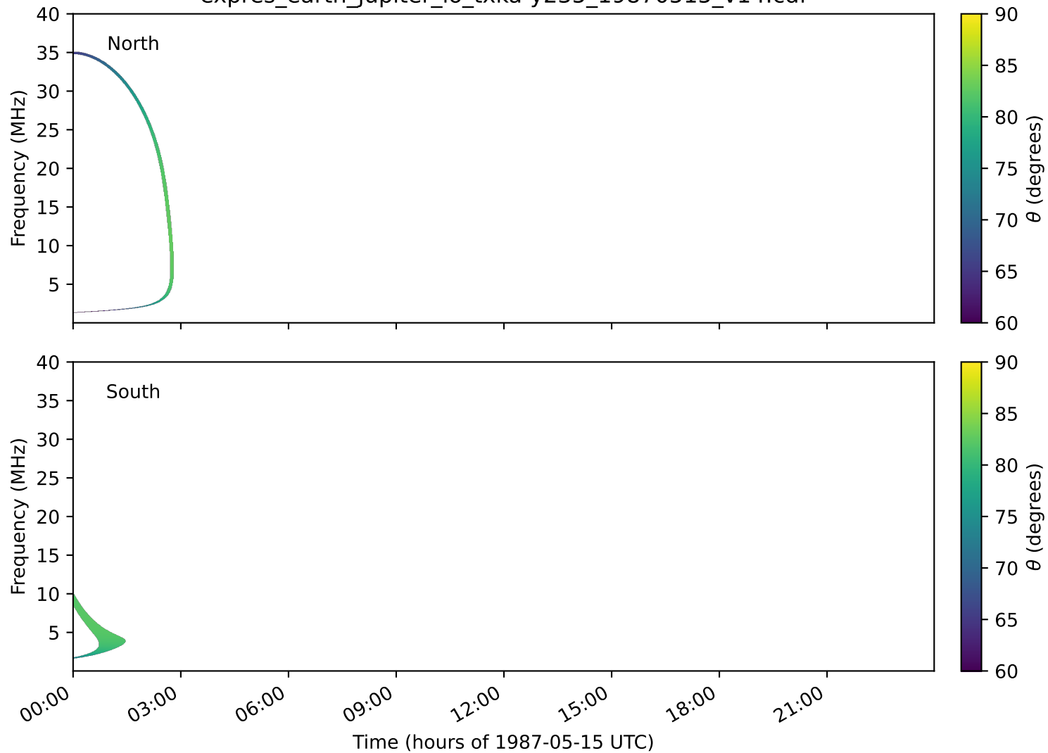
expres_earth_jupiter_io_txka-y235_19870515_v14.cdf
