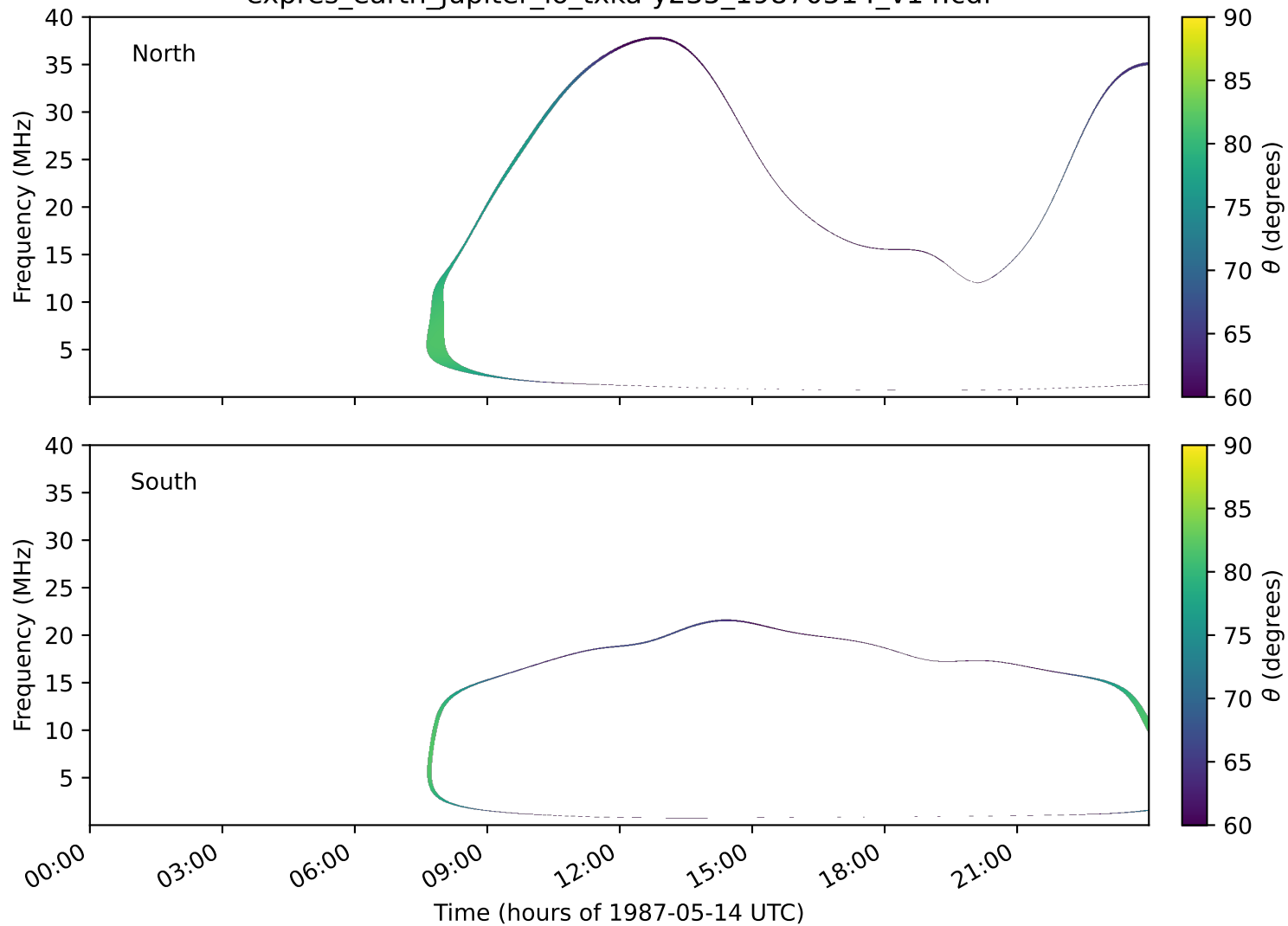
expres_earth_jupiter_io_txka-y235_19870514_v14.cdf
