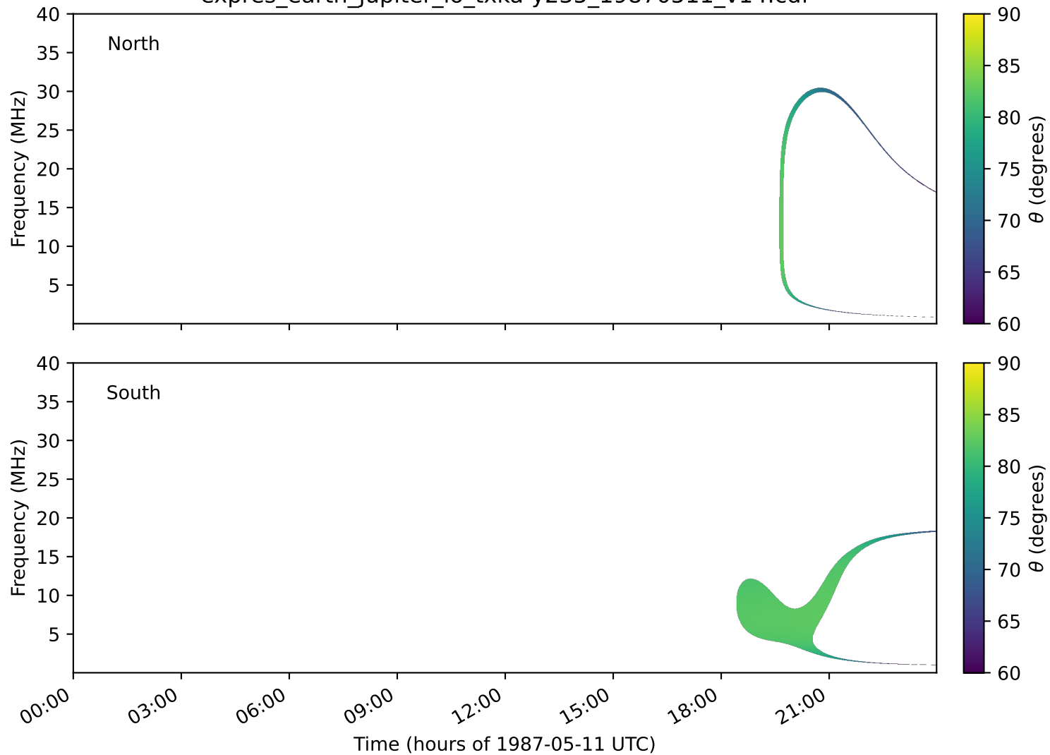
expres_earth_jupiter_io_txka-y235_19870511_v14.cdf
