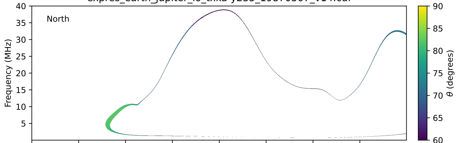
expres_earth_jupiter_io_txka-y235_19870507_v14.cdf
