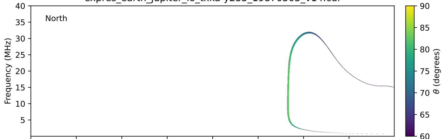
expres_earth_jupiter_io_txka-y235_19870503_v14.cdf
