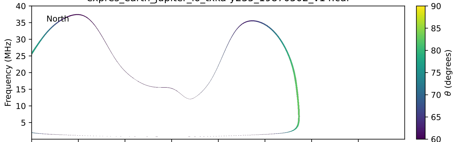
expres_earth_jupiter_io_txka-y235_19870502_v14.cdf
