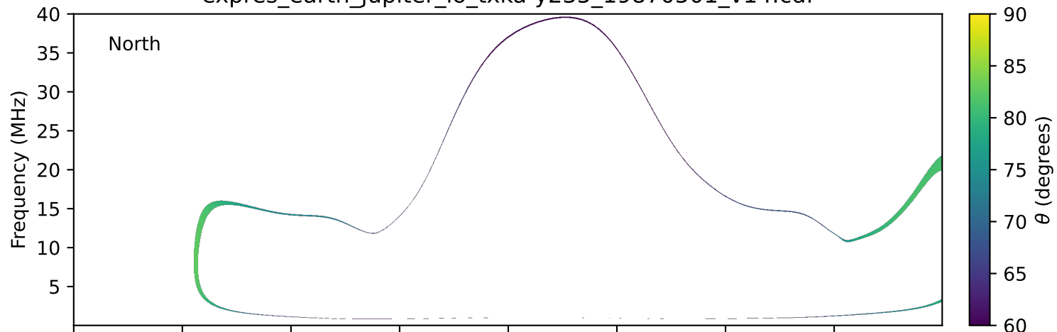
expres_earth_jupiter_io_txka-y235_19870501_v14.cdf
