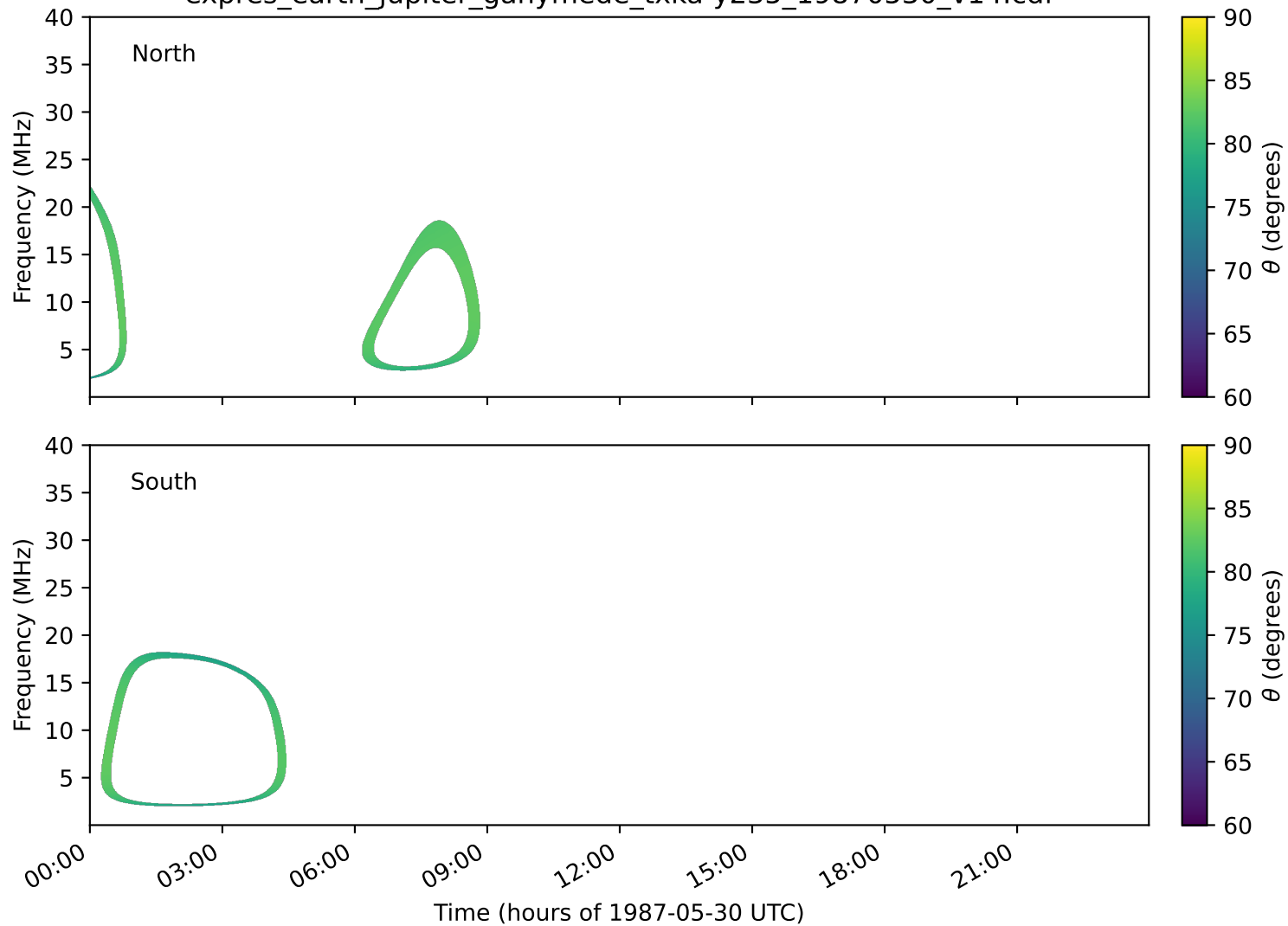
expres_earth_jupiter_ganymede_txka-y235_19870530_v14.cdf
