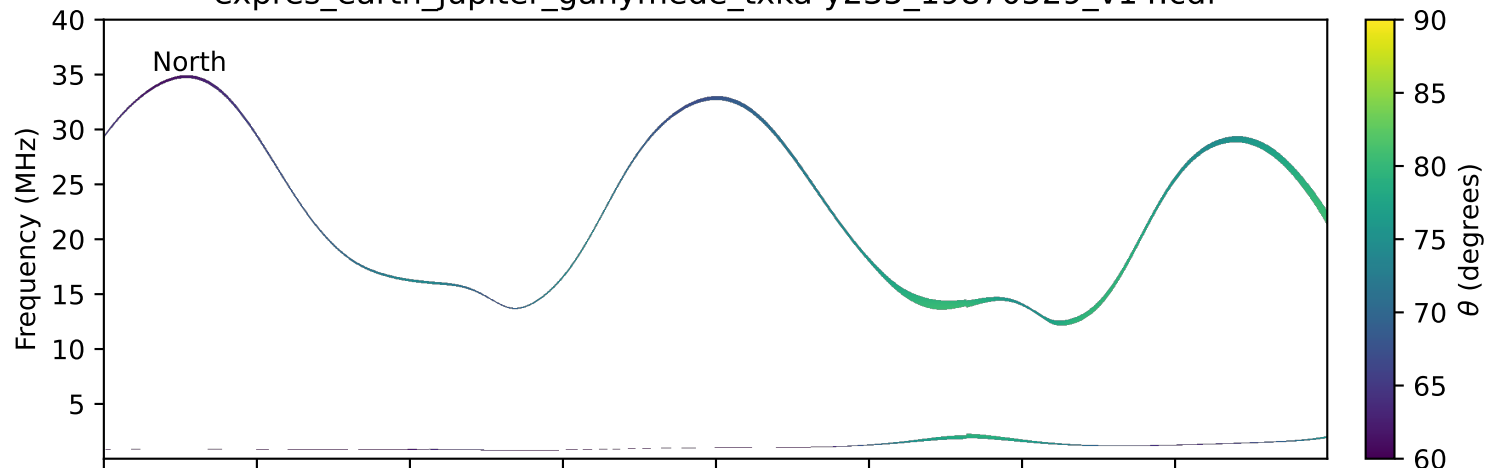
expres_earth_jupiter_ganymede_txka-y235_19870529_v14.cdf
