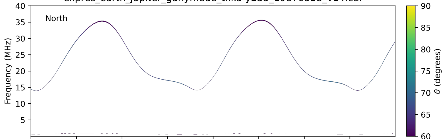
expres_earth_jupiter_ganymede_txka-y235_19870528_v14.cdf
