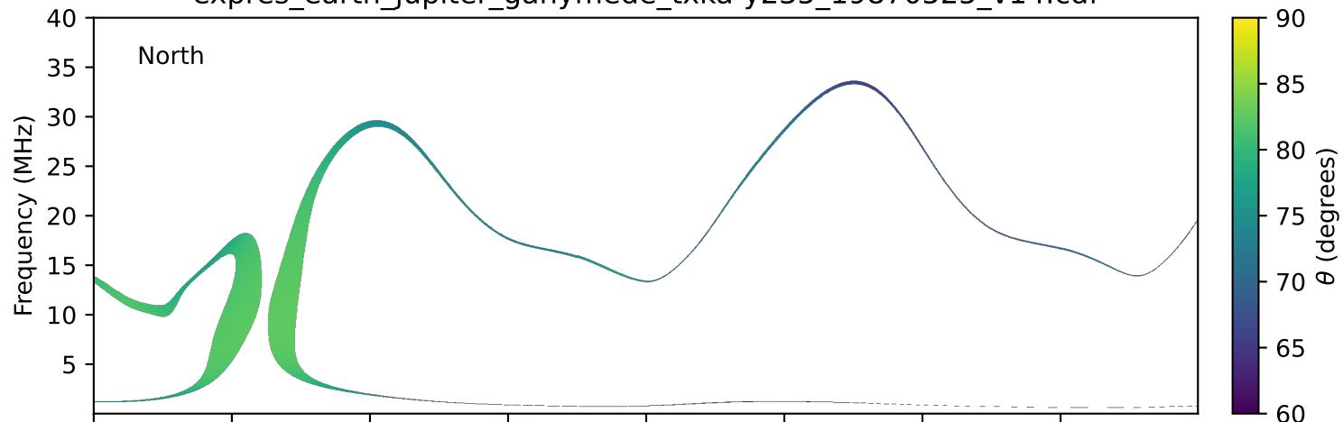
expres_earth_jupiter_ganymede_txka-y235_19870525_v14.cdf
