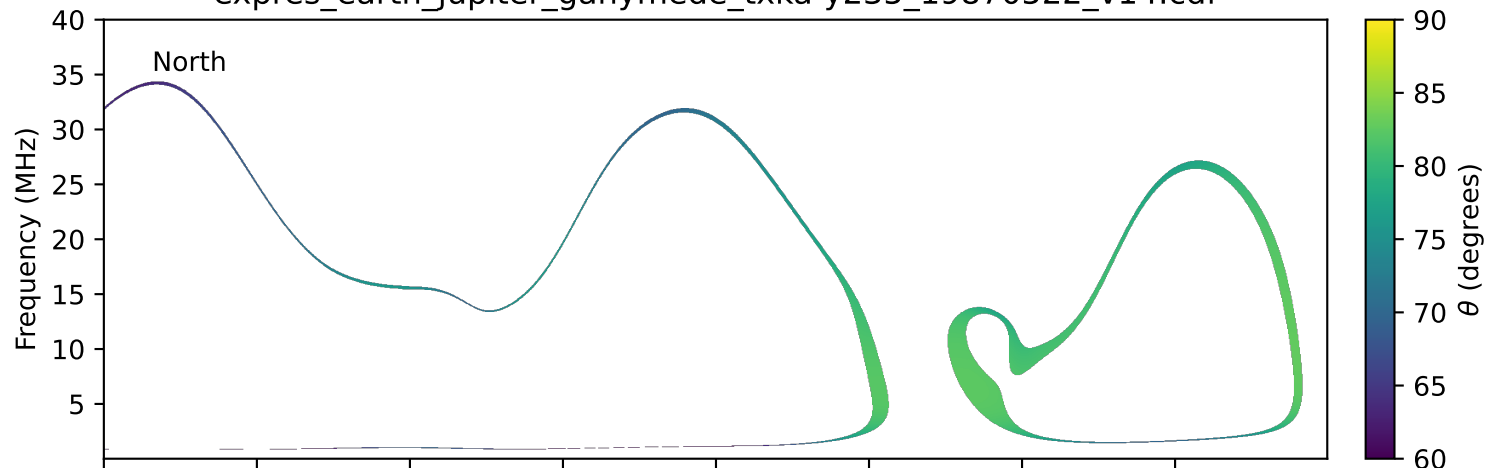
expres_earth_jupiter_ganymede_txka-y235_19870522_v14.cdf
