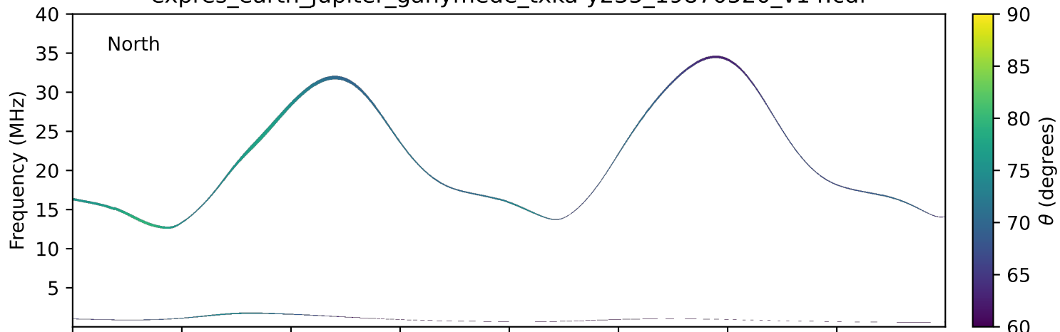
expres_earth_jupiter_ganymede_txka-y235_19870520_v14.cdf
