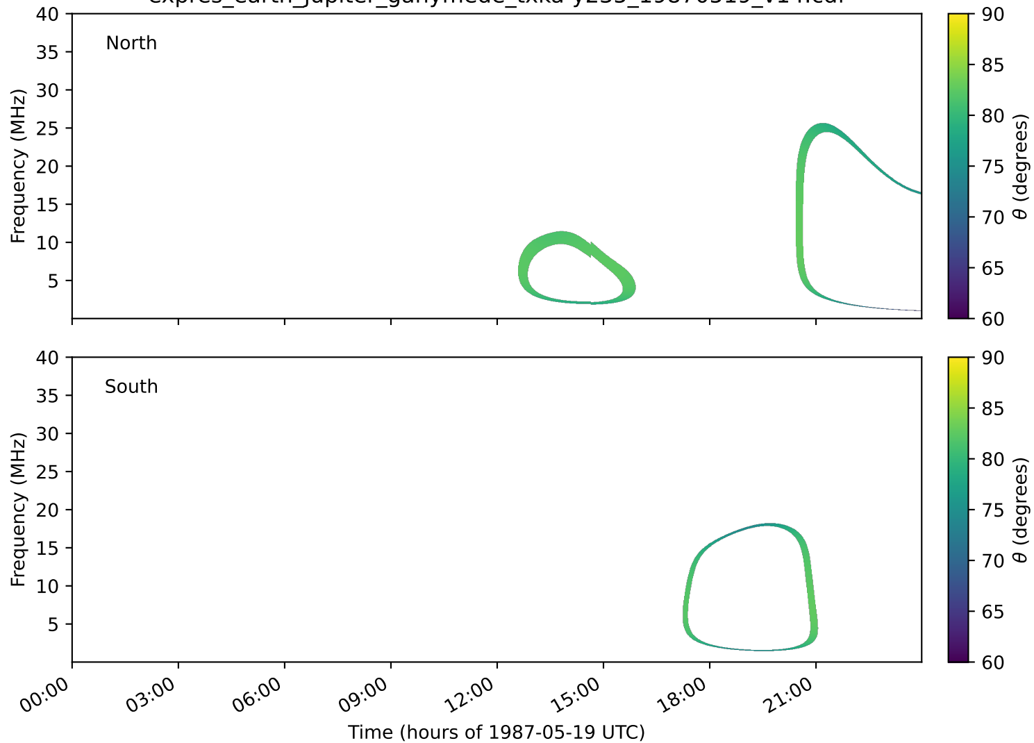
expres_earth_jupiter_ganymede_txka-y235_19870519_v14.cdf
