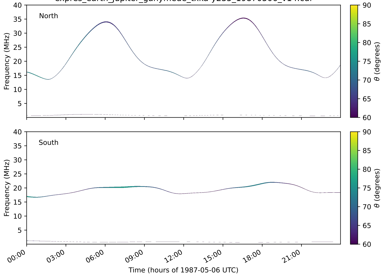
expres_earth_jupiter_ganymede_txka-y235_19870506_v14.cdf
