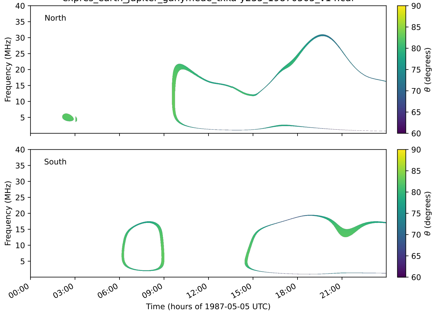
expres_earth_jupiter_ganymede_txka-y235_19870505_v14.cdf
