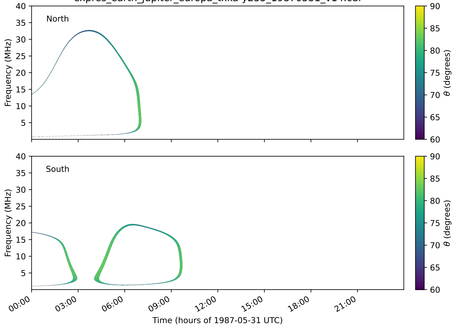
expres_earth_jupiter_europa_txka-y235_19870531_v14.cdf
