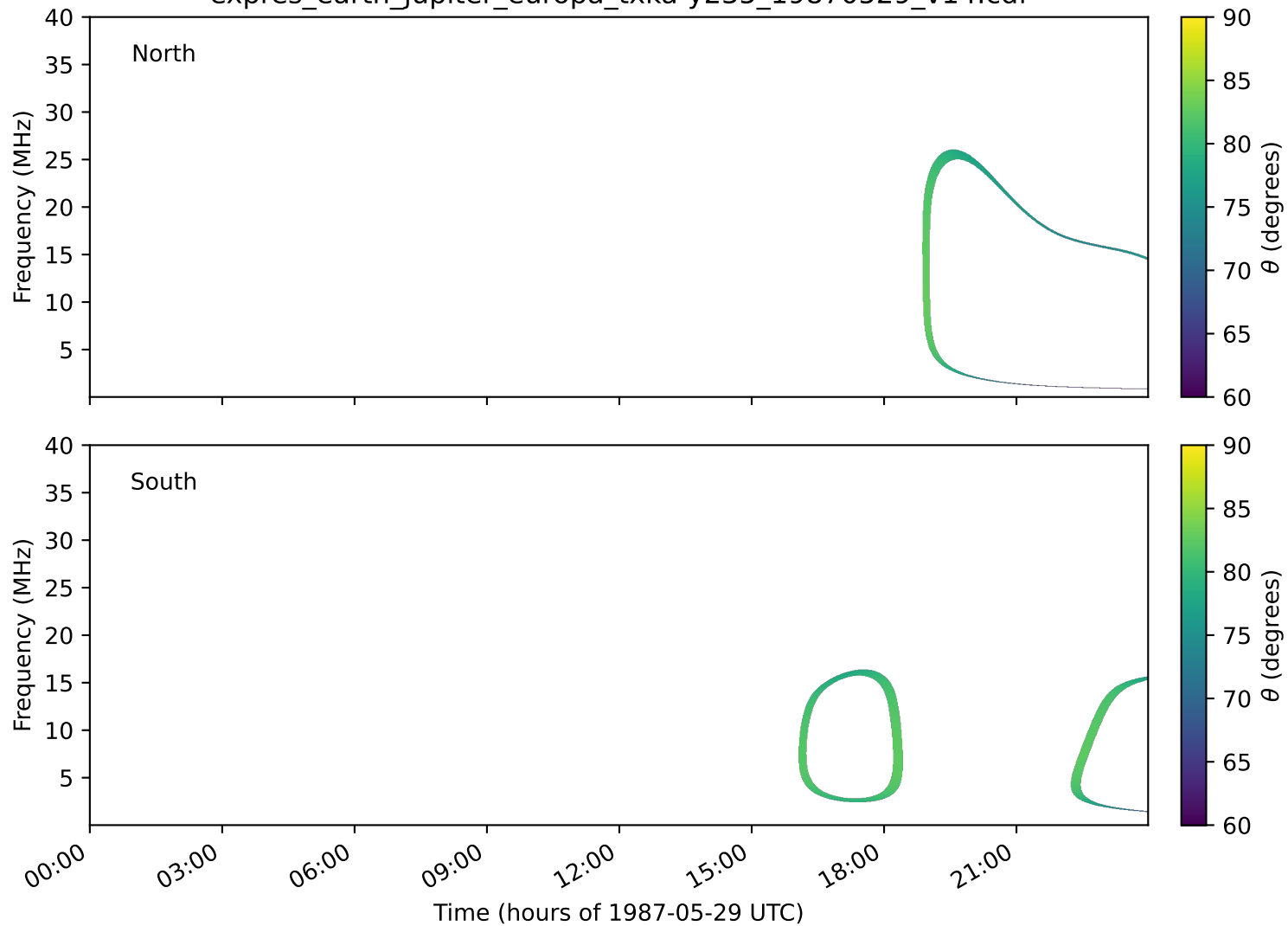
expres_earth_jupiter_europa_txka-y235_19870529_v14.cdf
