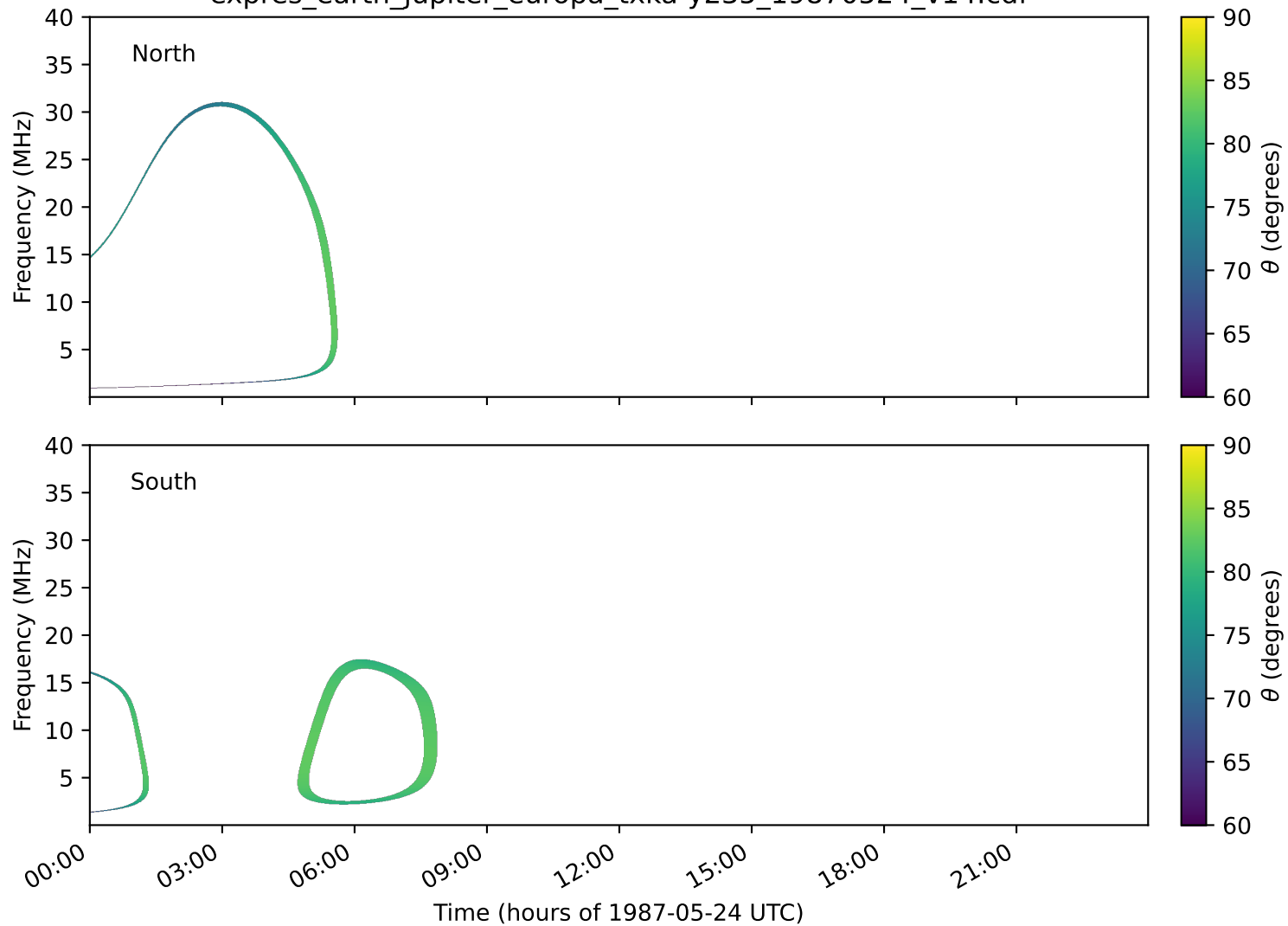
expres_earth_jupiter_europa_txka-y235_19870524_v14.cdf
