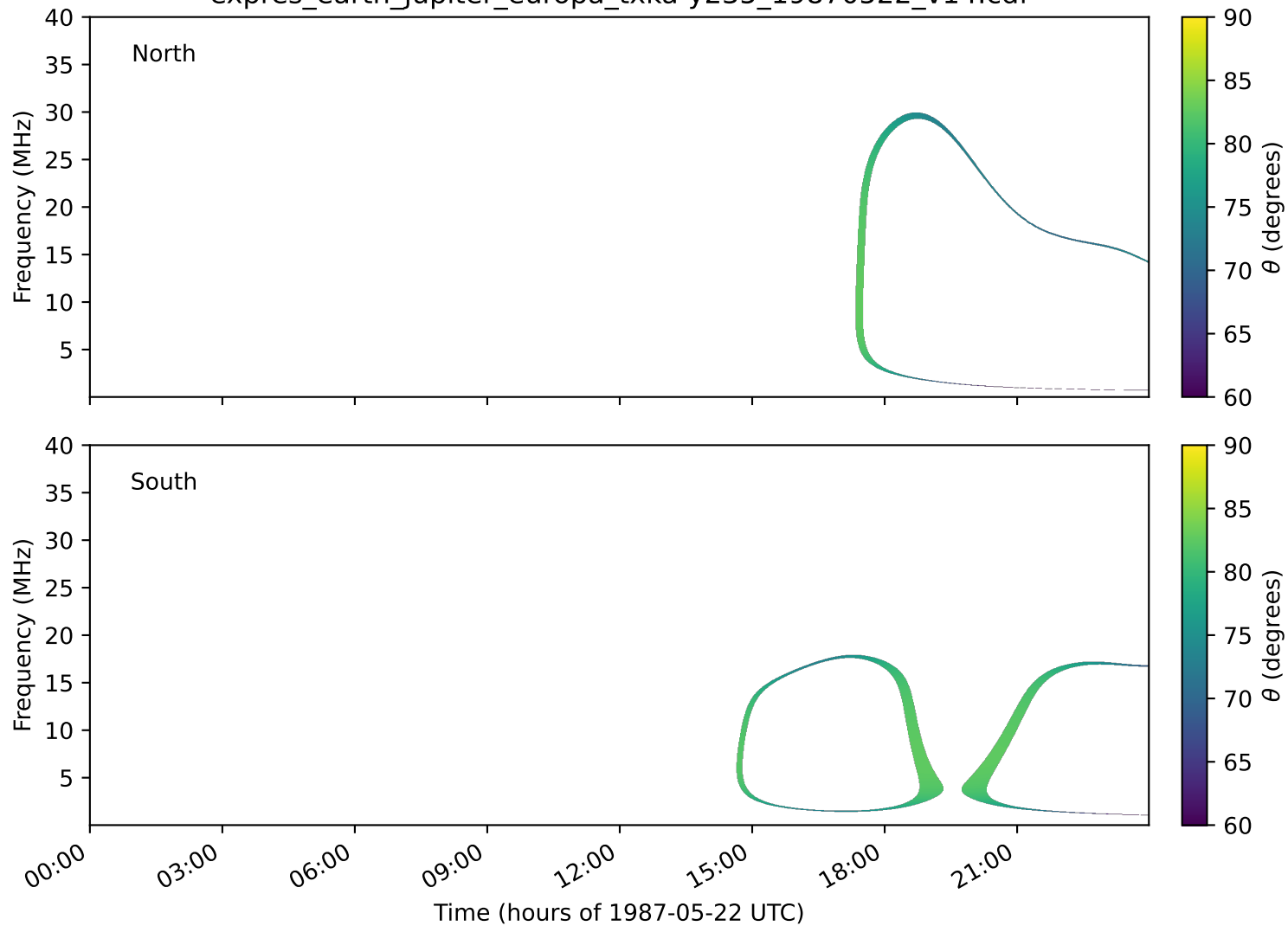
expres_earth_jupiter_europa_txka-y235_19870522_v14.cdf
