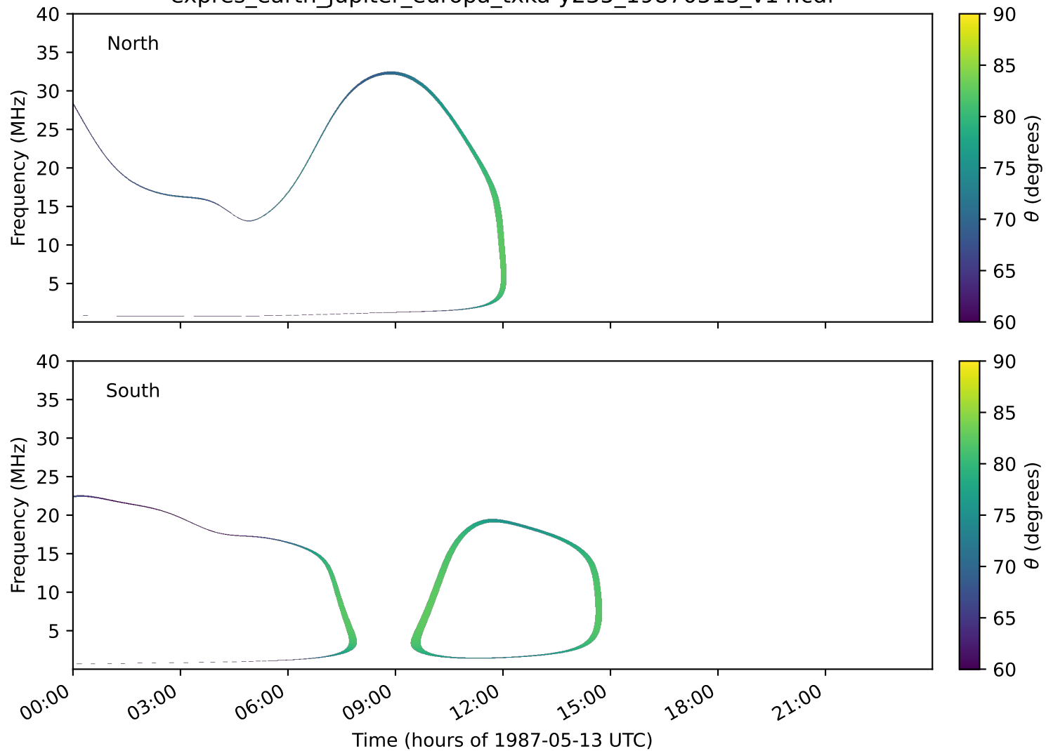
expres_earth_jupiter_europa_txka-y235_19870513_v14.cdf
