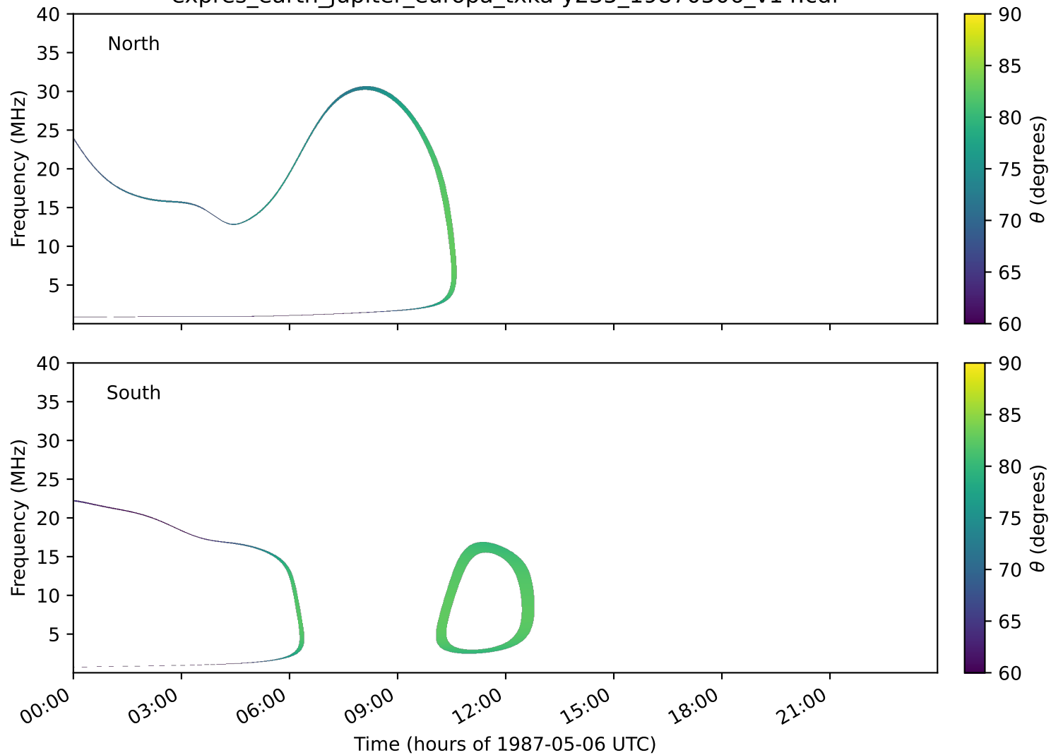
expres_earth_jupiter_europa_txka-y235_19870506_v14.cdf
