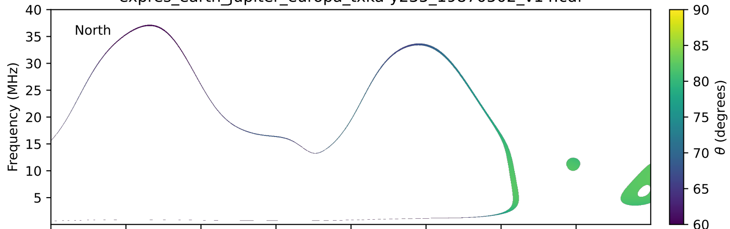
expres_earth_jupiter_europa_txka-y235_19870502_v14.cdf
