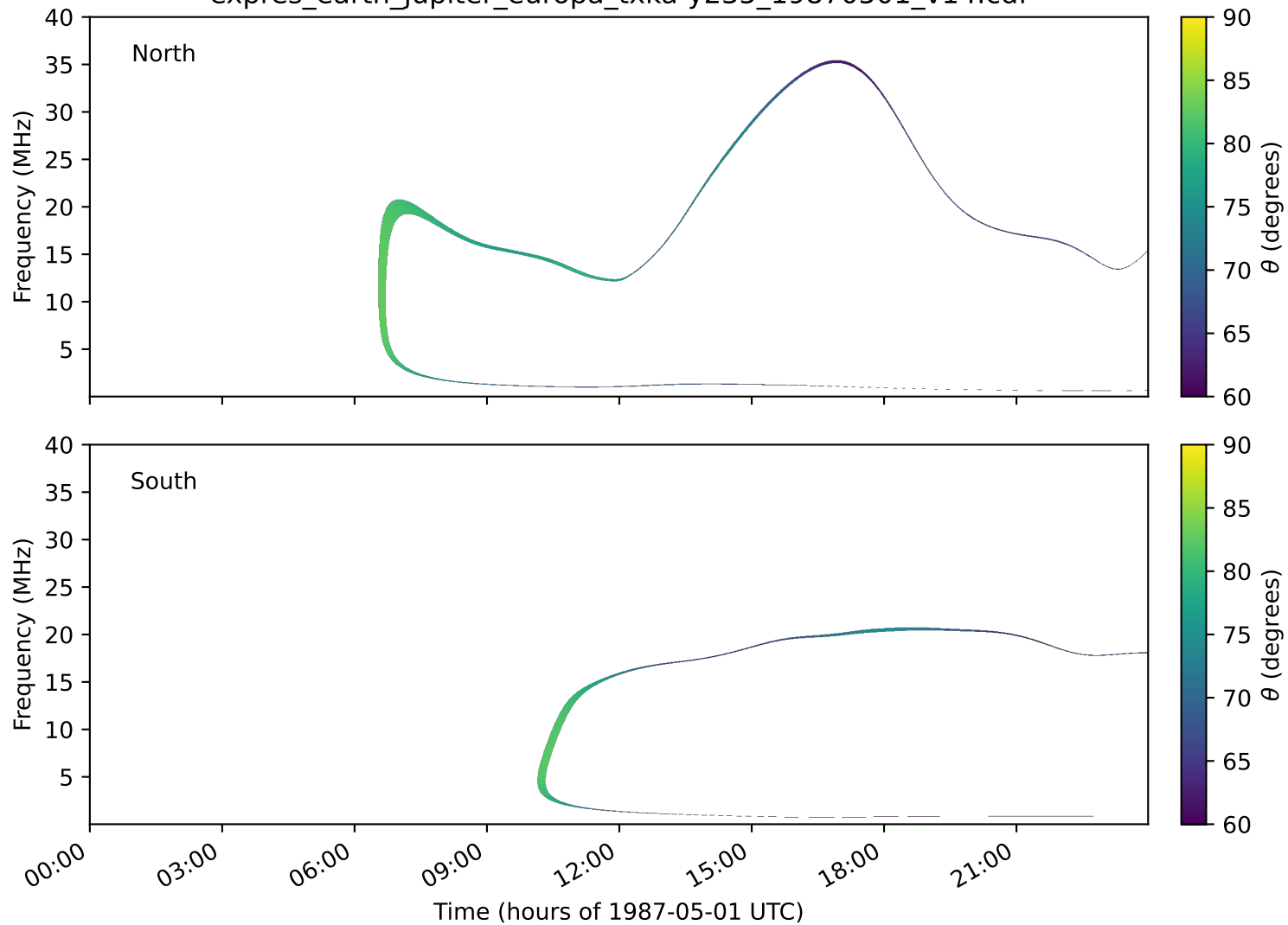
expres_earth_jupiter_europa_txka-y235_19870501_v14.cdf
